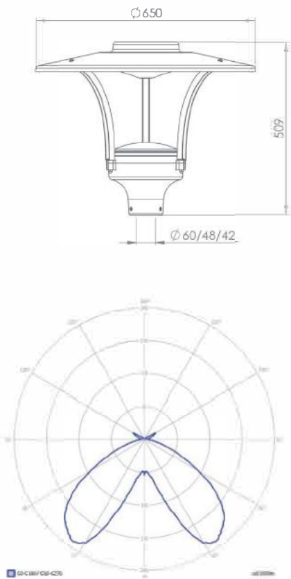
Promenade Led Indirect 30
