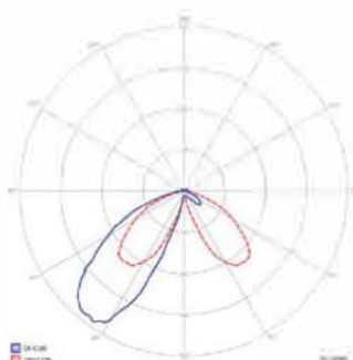
Promenade Led ASM 30
