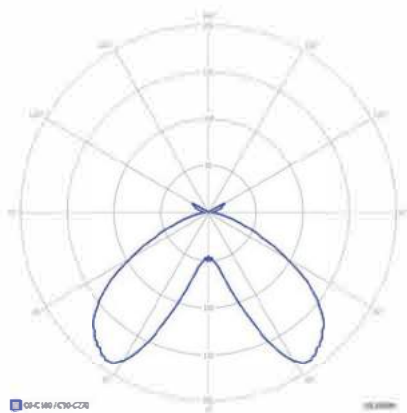
Promenade Led Indirect 45
